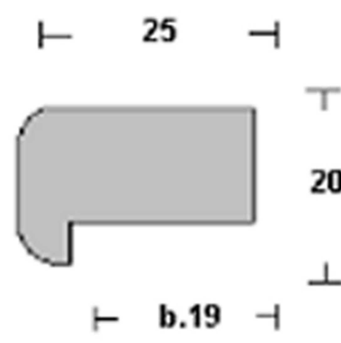
Art. 36 - 1D 25 x 20
